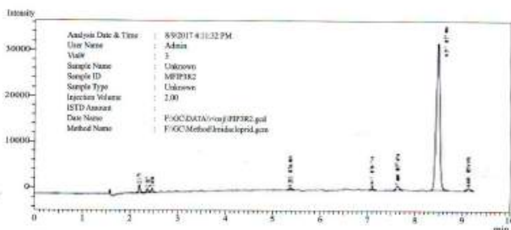
Fig. 2. Chromatogram of dissipation kinetics of Imidacloprid on country bean after 1 DAT.
