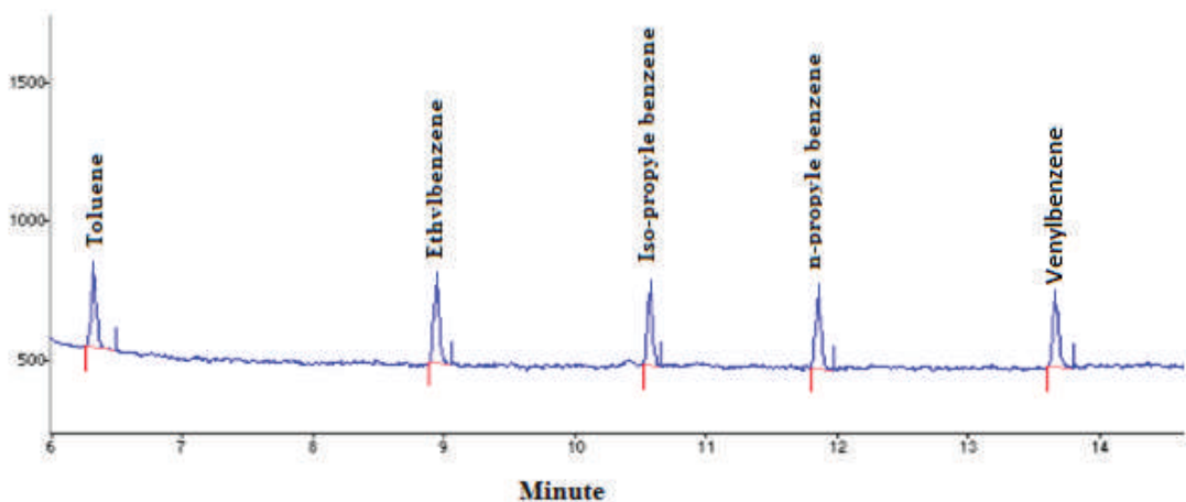
Fig. 3. GC-FID chromatogram of a 1.0 \mu\text{g/mL} standard solution of the five test compounds
