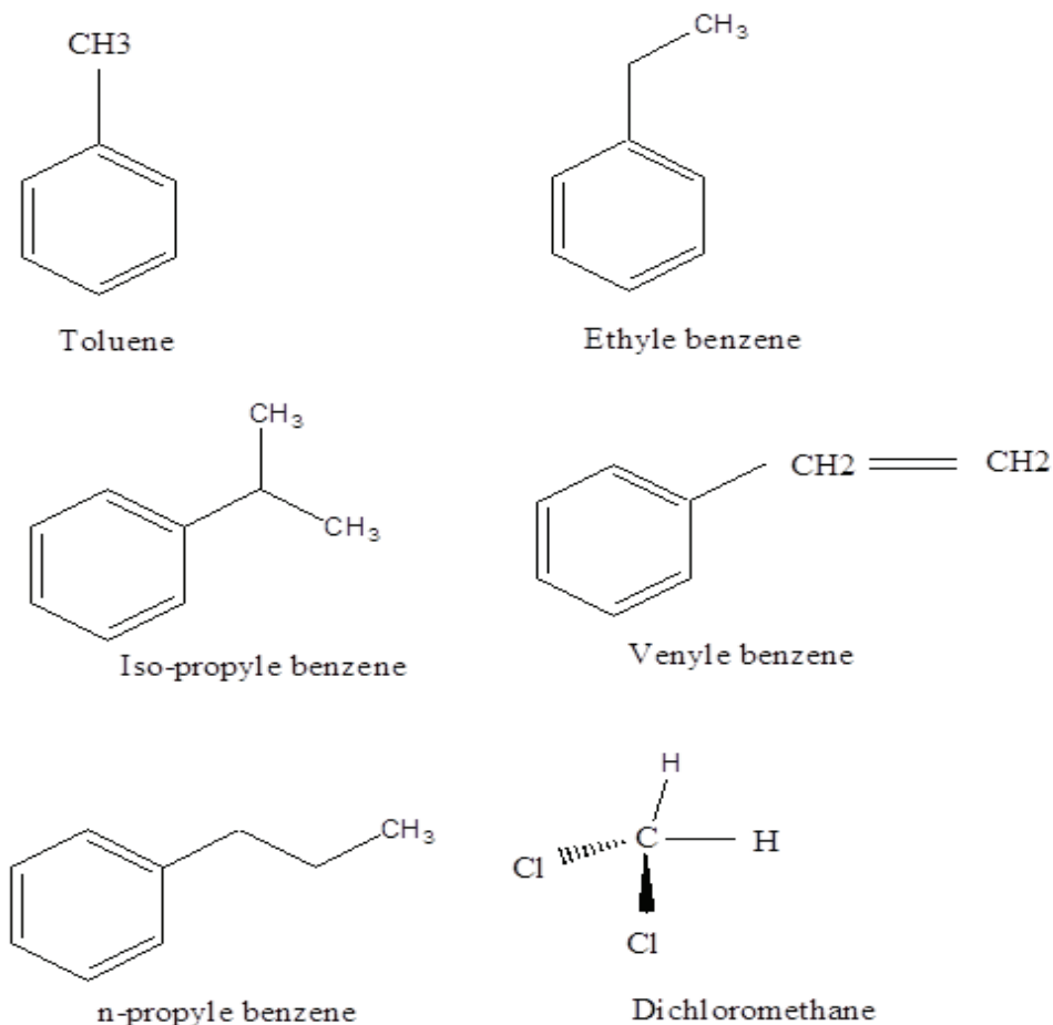
Fig. 2. Chemical structures of the standards and reagents
